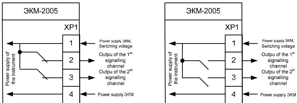
For variant of execution of Signaling instruments III
