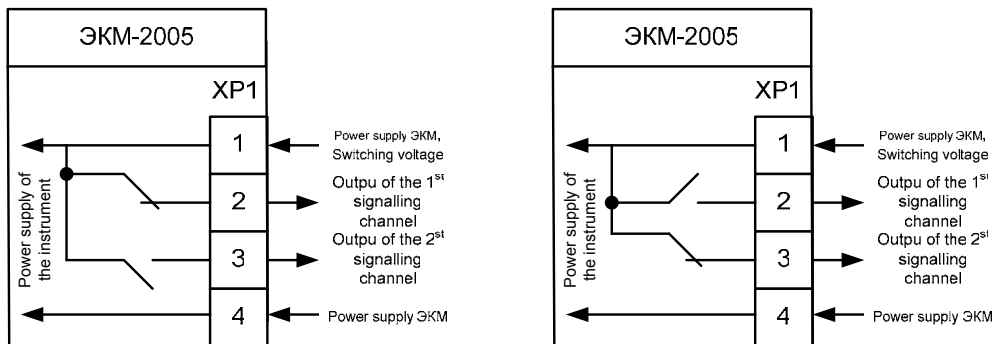
For variant of execution of Signaling instruments V
